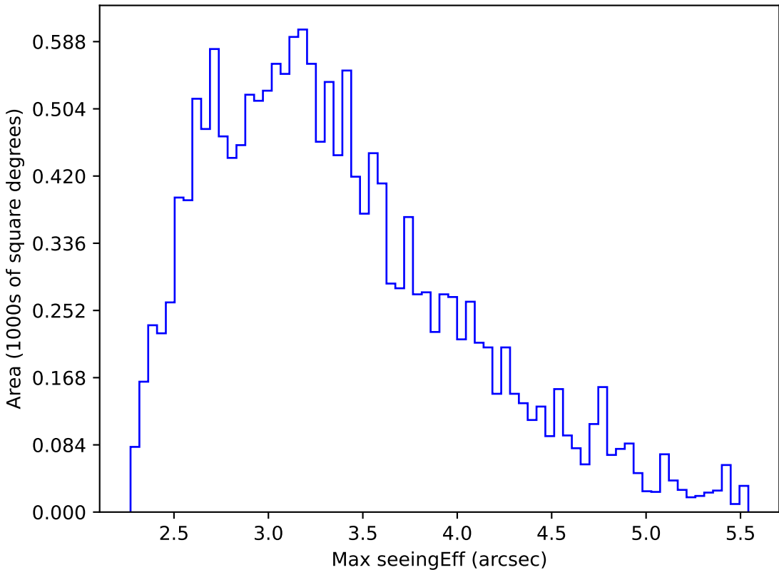
too_elab_r128_d2_griz_v3.4_10yrs WFD all bands: Max seeingEff
