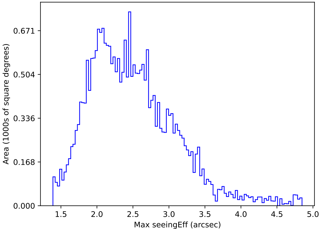
too_elab_r128_d2_griz_v3.4_10yrs All sky z band: Max seeingEff
