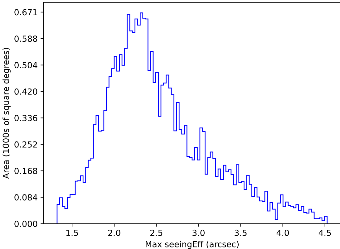
too_elab_r128_d2_griz_v3.4_10yrs All sky u band: Max seeingEff
