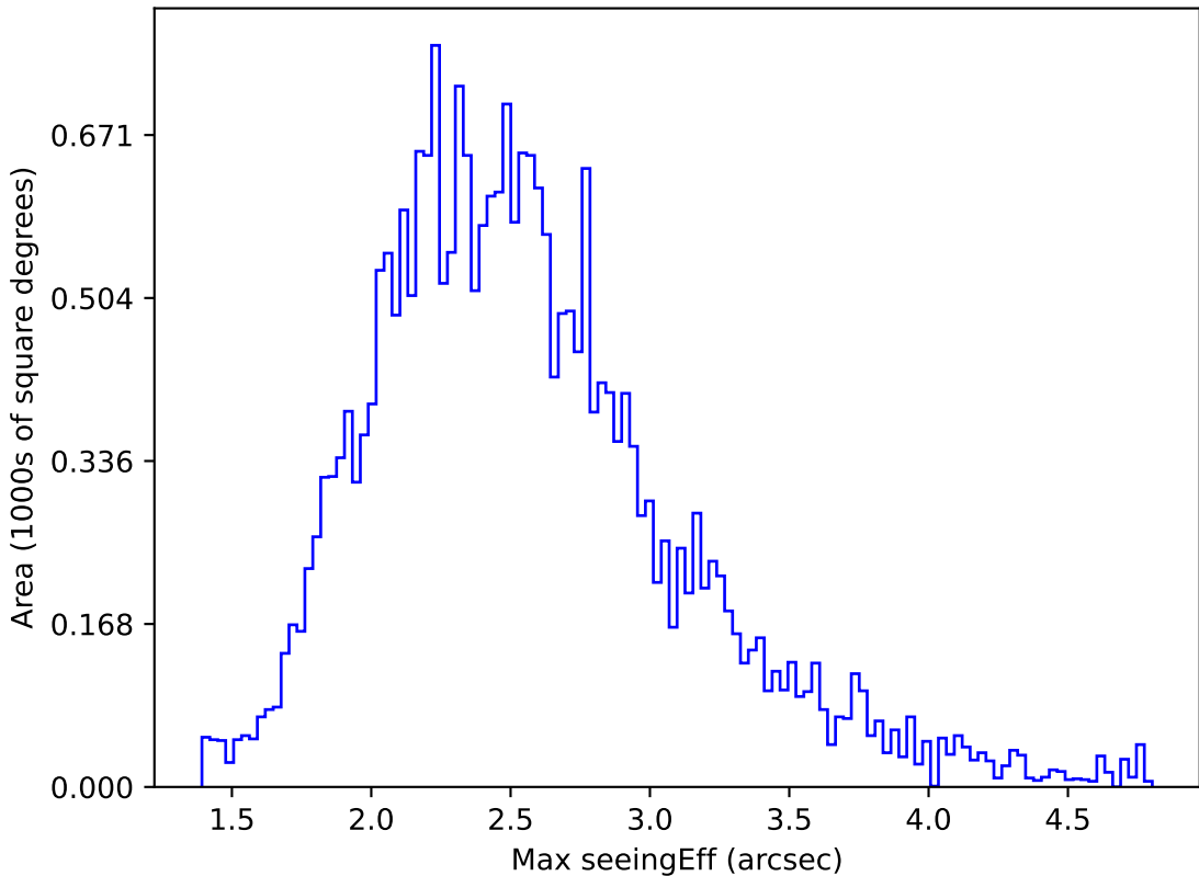
too_elab_r128_d2_griz_v3.4_10yrs All sky i band: Max seeingEff
