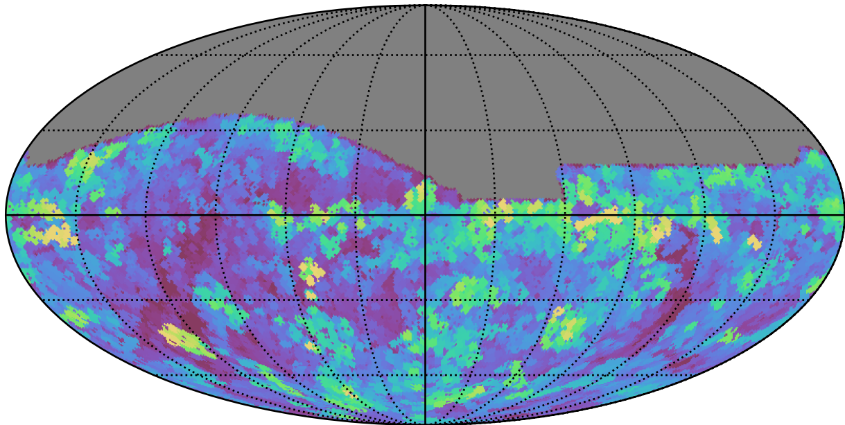
too_elab_r128_d2_griz_v3.4_10yrs All sky g band: Max seeingEff
