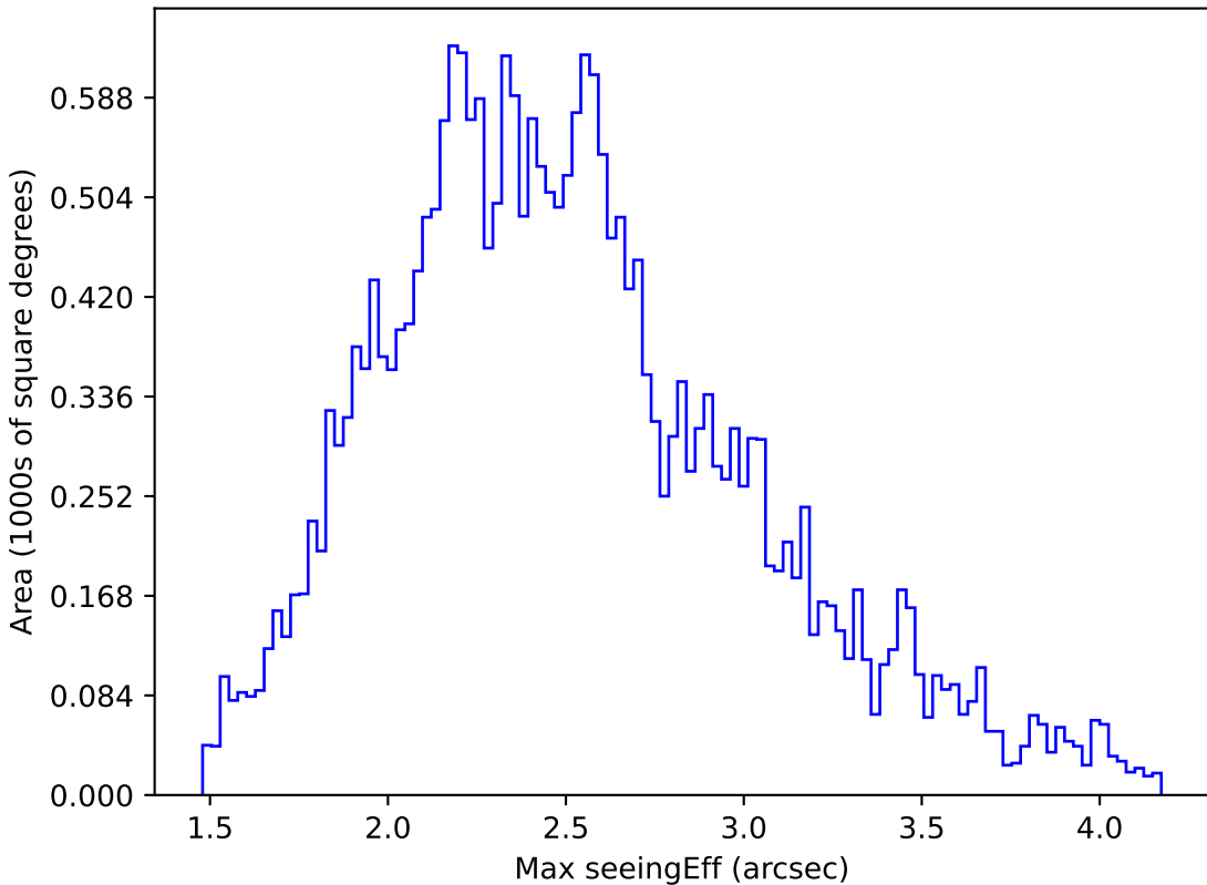
too_elab_r128_d2_griz_v3.4_10yrs All sky g band: Max seeingEff
