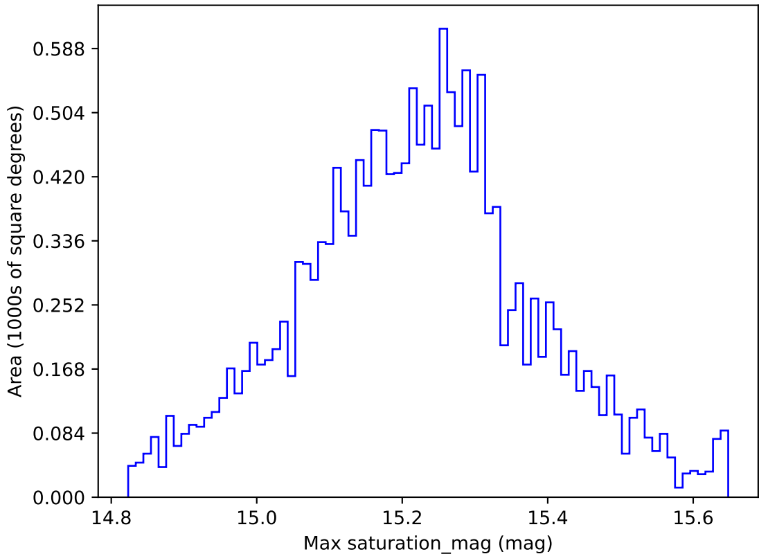
too_elab_r128_d2_griz_v3.4_10yrs WFD z band: Max saturation_mag
