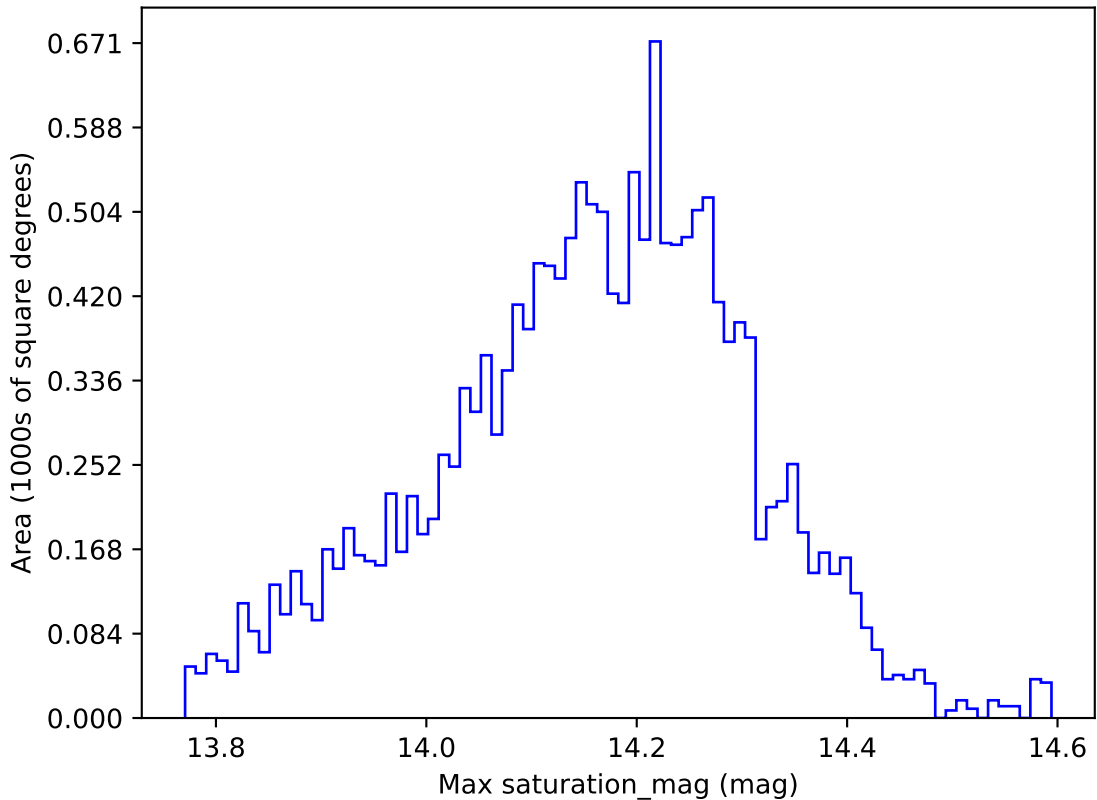
too_elab_r128_d2_griz_v3.4_10yrs WFD y band: Max saturation_mag
