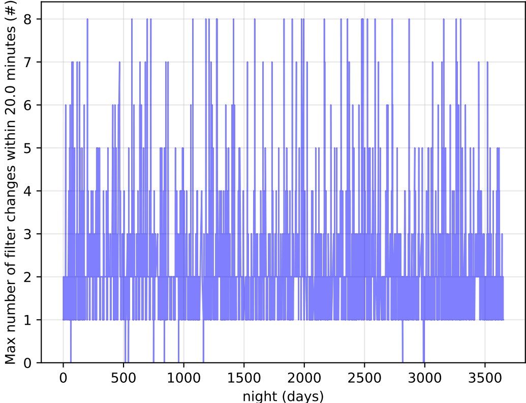
too_elab_r128_d2_griz_v3.4_10yrs Per Night: Max number of filter changes within 20.0 minutes
