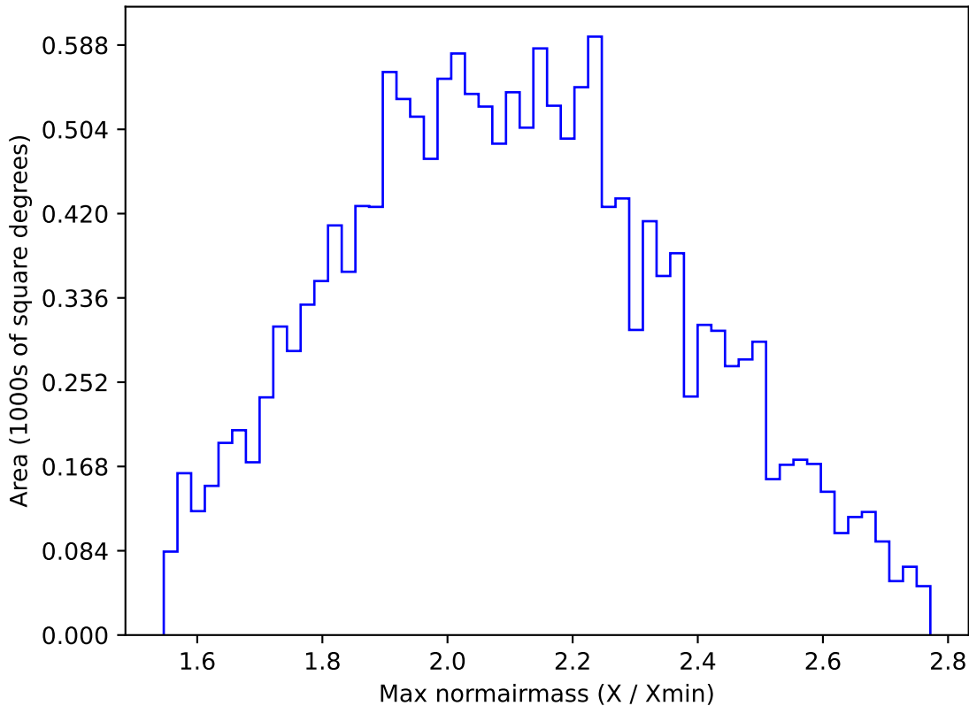
too_elab_r128_d2_griz_v3.4_10yrs WFD y band: Max normairmass
