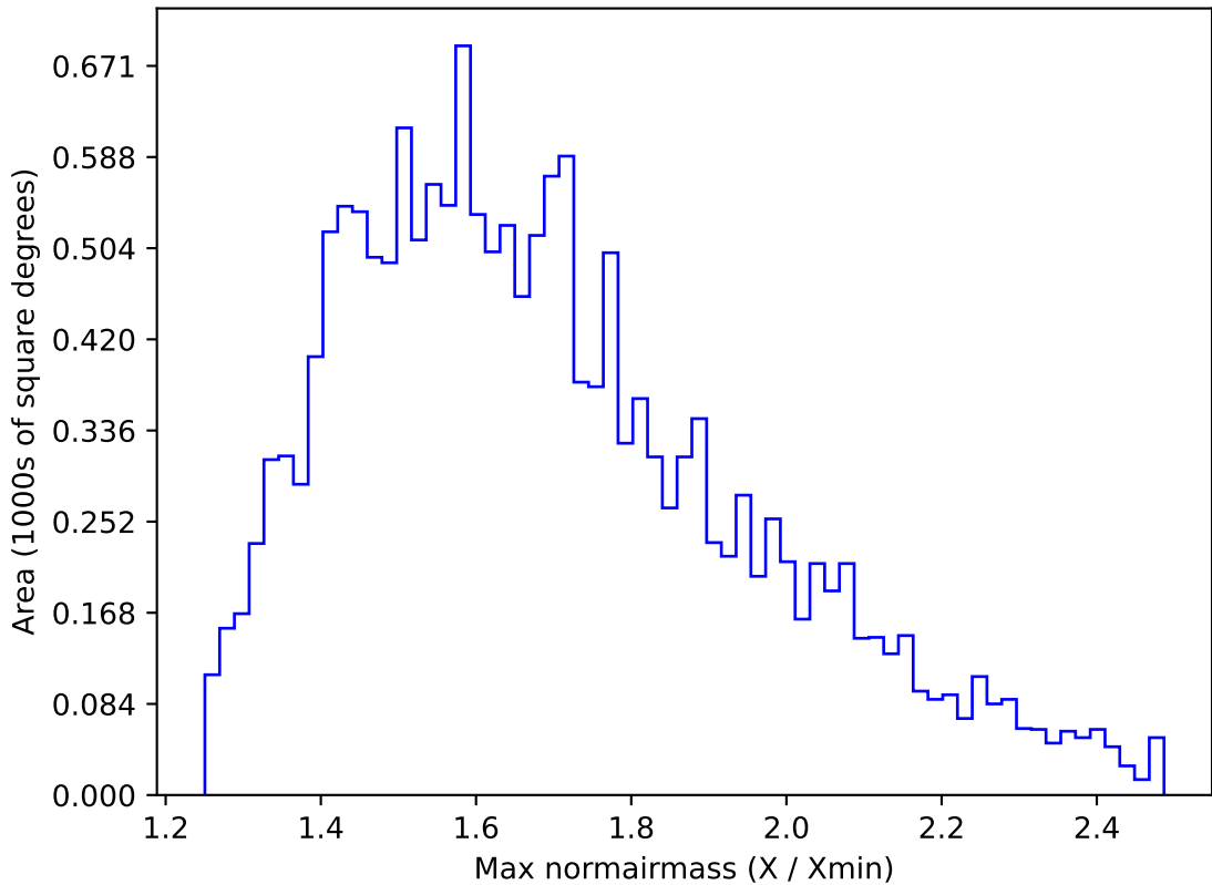
too_elab_r128_d2_griz_v3.4_10yrs WFD u band: Max normairmass
