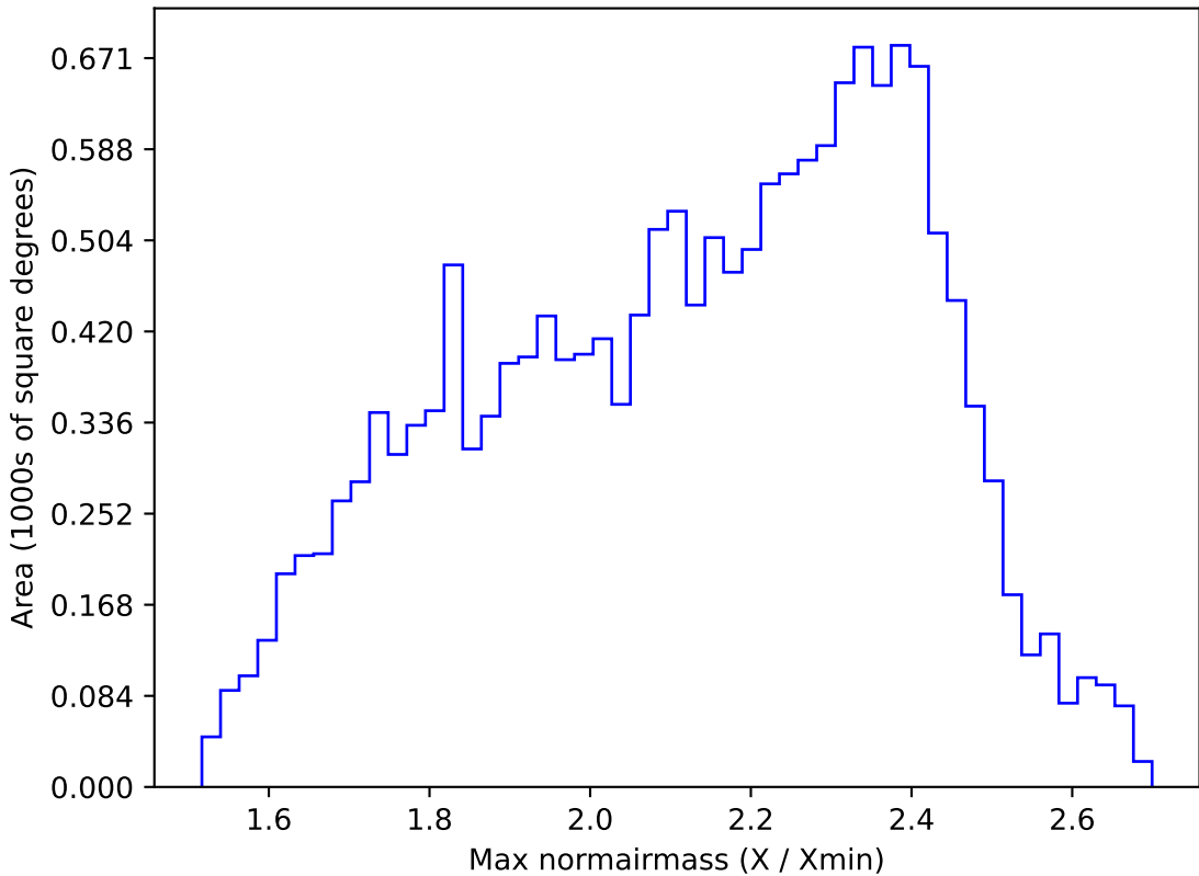
too_elab_r128_d2_griz_v3.4_10yrs WFD r band: Max normairmass
