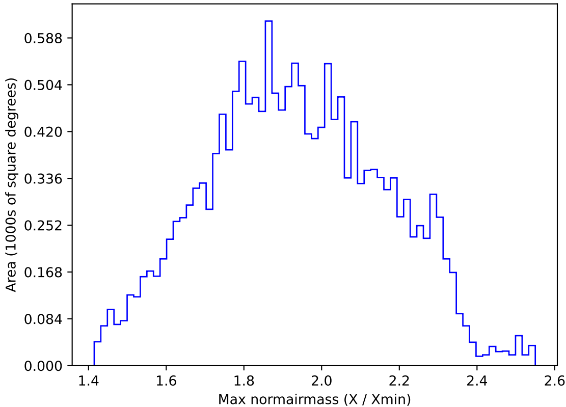
too_elab_r128_d2_griz_v3.4_10yrs WFD g band: Max normairmass
