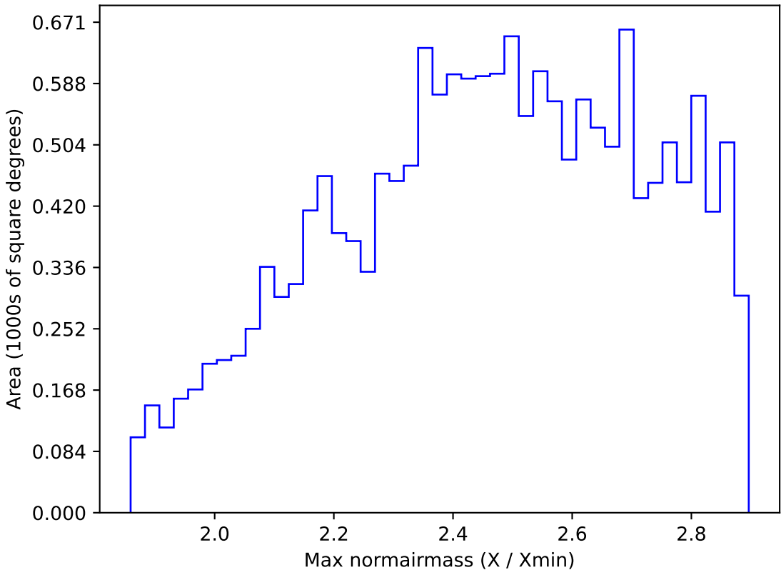
too_elab_r128_d2_griz_v3.4_10yrs WFD all bands: Max normairmass
