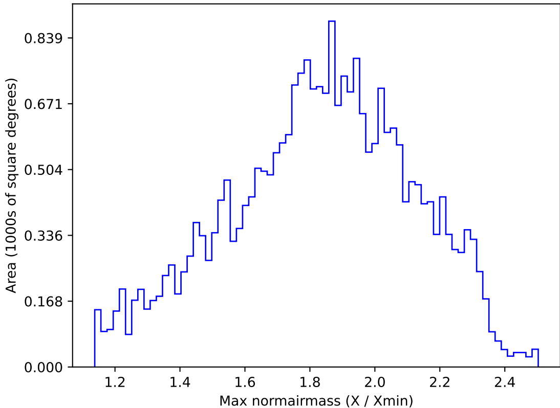
too_elab_r128_d2_griz_v3.4_10yrs All sky g band: Max normairmass
