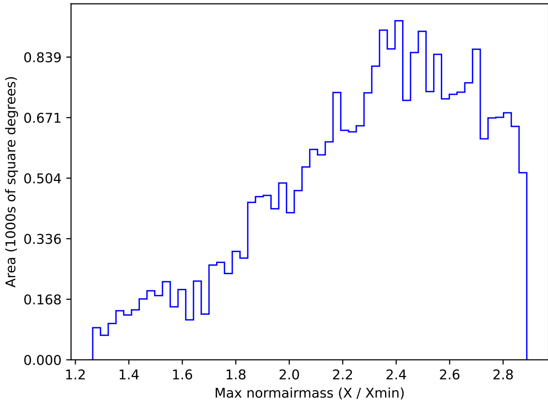
too_elab_r128_d2_griz_v3.4_10yrs All sky all bands: Max normairmass
