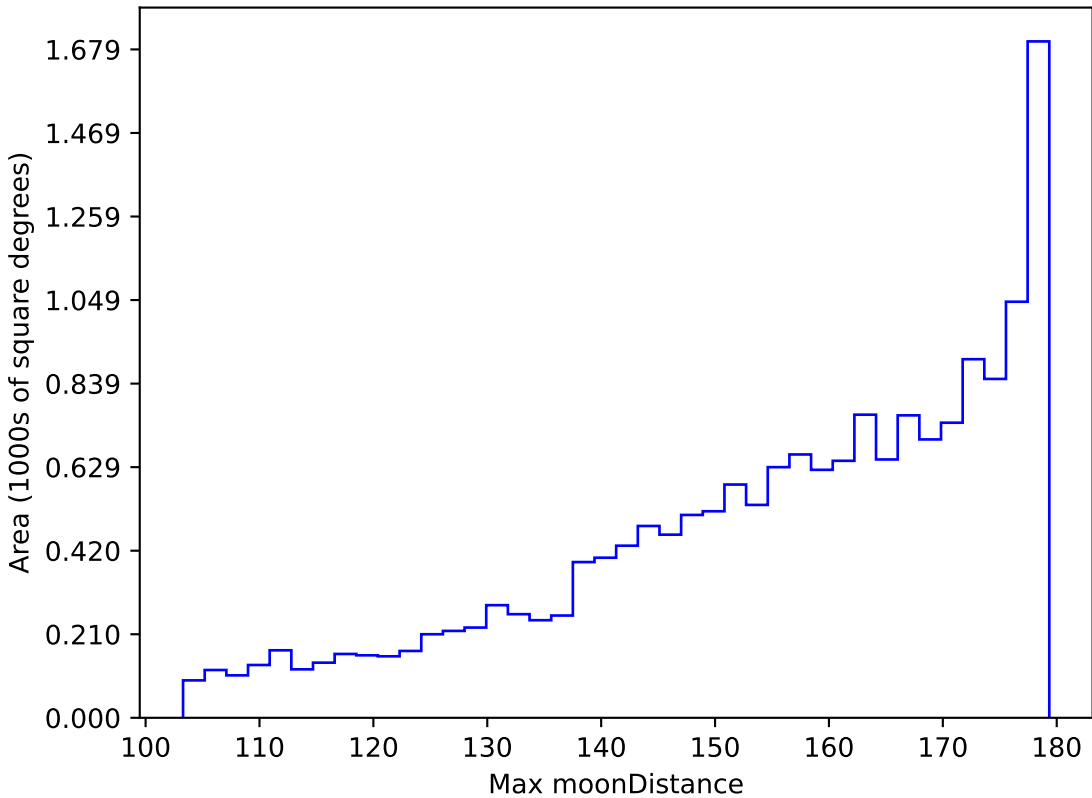
too_elab_r128_d2_griz_v3.4_10yrs WFD r band: Max moonDistance
