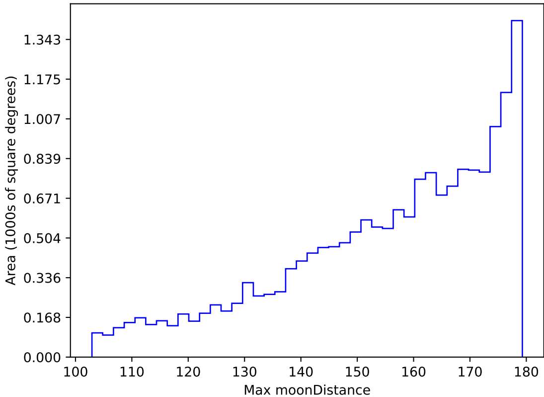
too_elab_r128_d2_griz_v3.4_10yrs WFD i band: Max moonDistance
