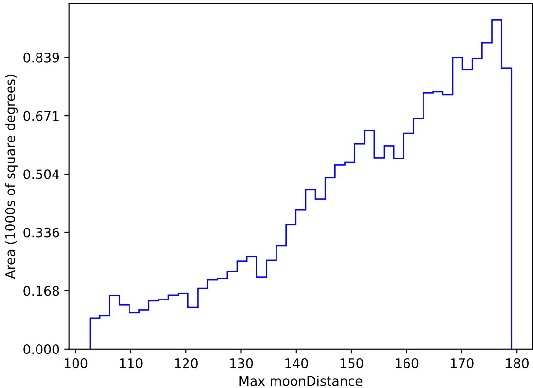
too_elab_r128_d2_griz_v3.4_10yrs WFD g band: Max moonDistance
