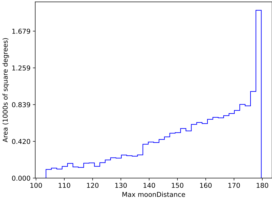
too_elab_r128_d2_griz_v3.4_10yrs WFD all bands: Max moonDistance
