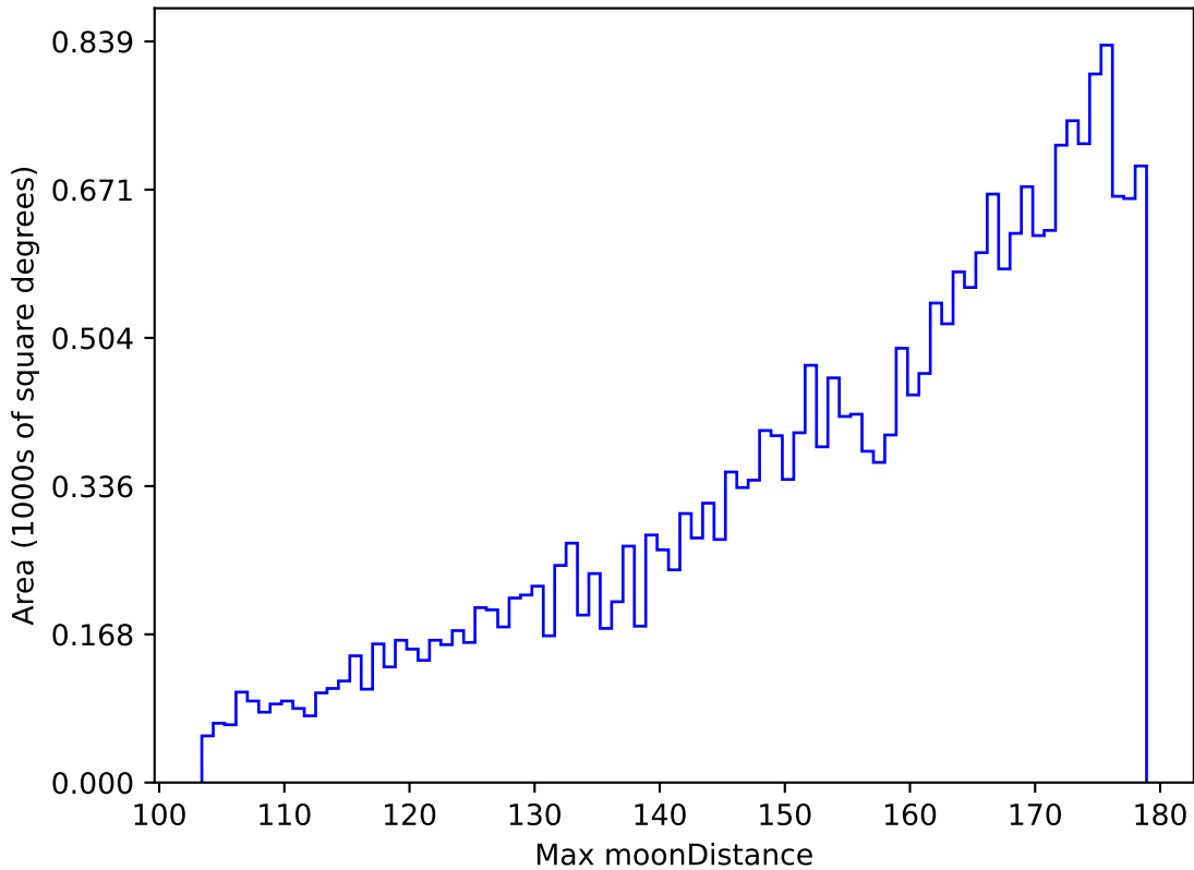
too_elab_r128_d2_griz_v3.4_10yrs All sky g band: Max moonDistance
