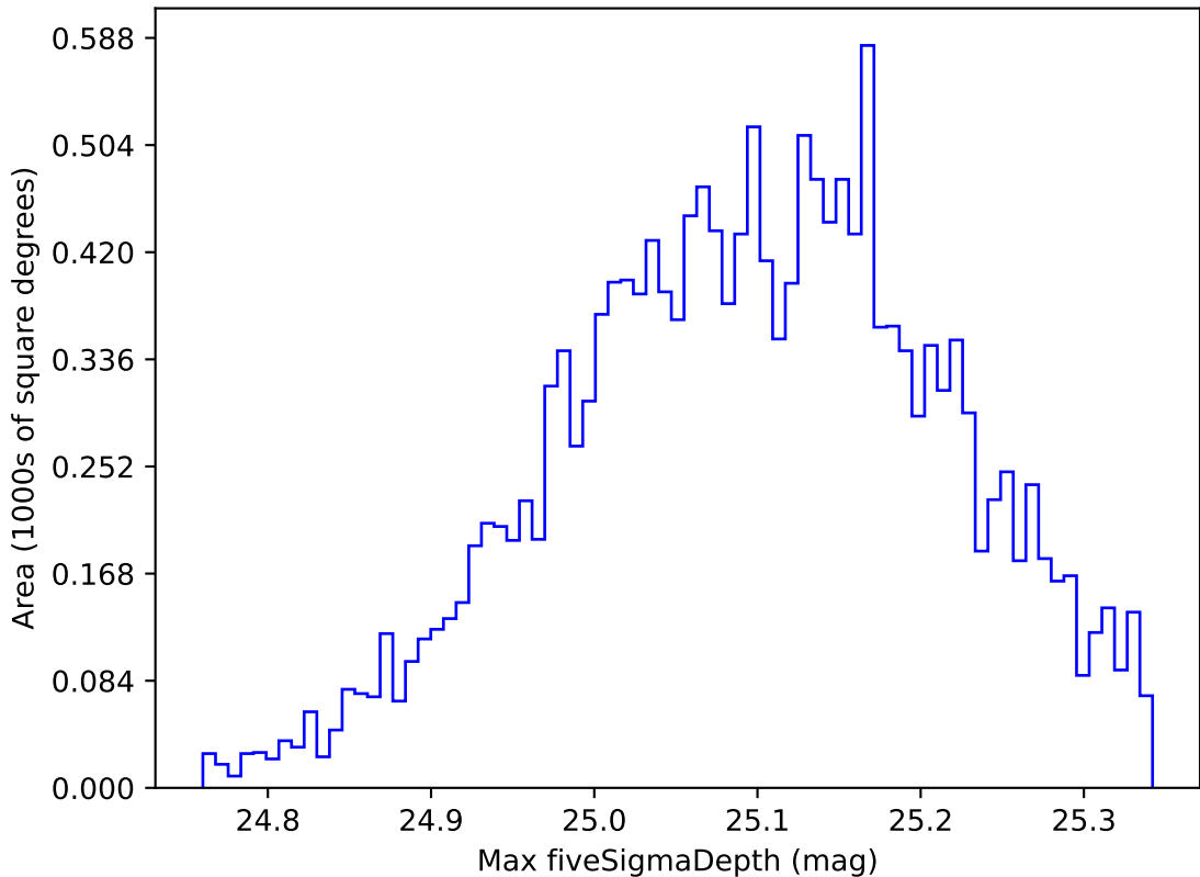
too_elab_r128_d2_griz_v3.4_10yrs WFD g band: Max fiveSigmaDepth
