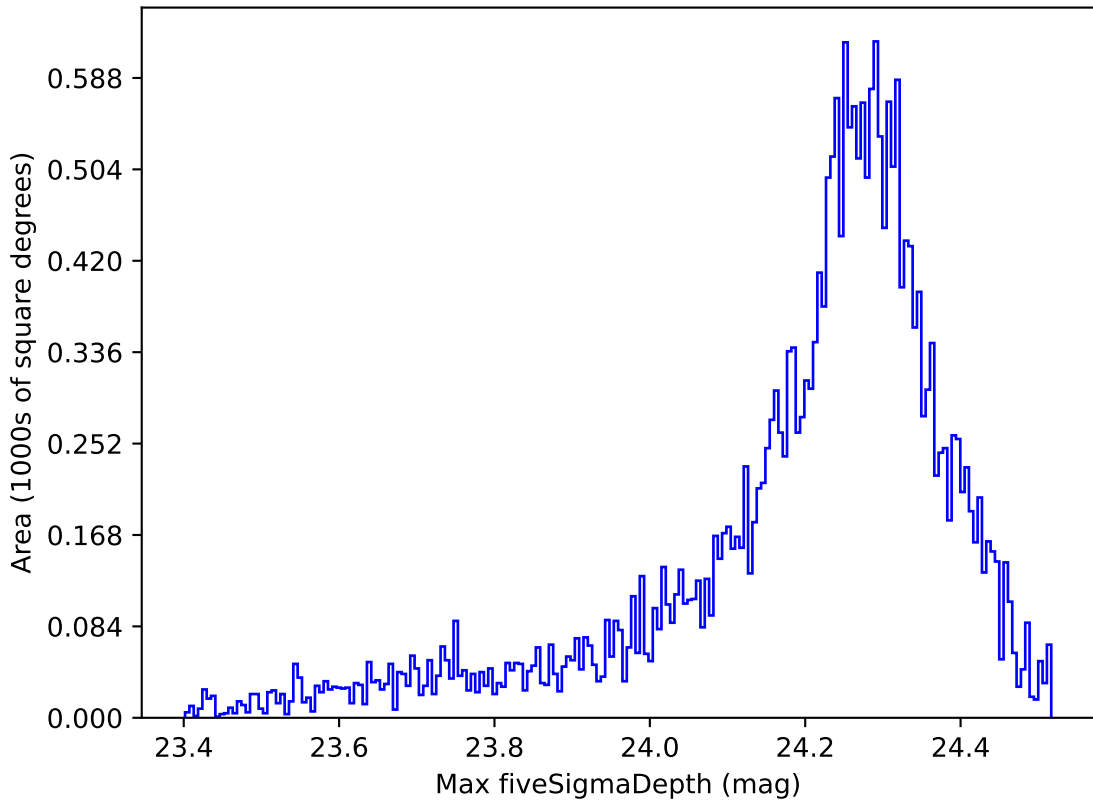
too_elab_r128_d2_griz_v3.4_10yrs All sky i band: Max fiveSigmaDepth
