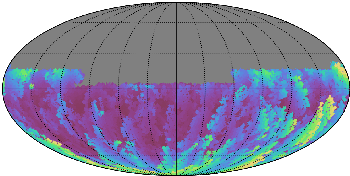
too_elab_r128_d2_griz_v3.4_10yrs Yr 1 u band: Max airmass
