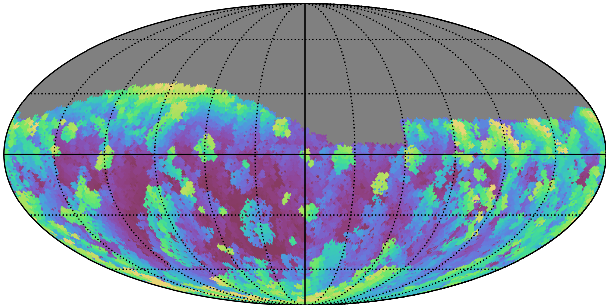
too_elab_r128_d2_griz_v3.4_10yrs Yr 1 g band: Max airmass
