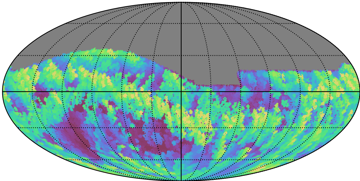
too_elab_r128_d2_griz_v3.4_10yrs Yr 1 all bands: Max airmass
