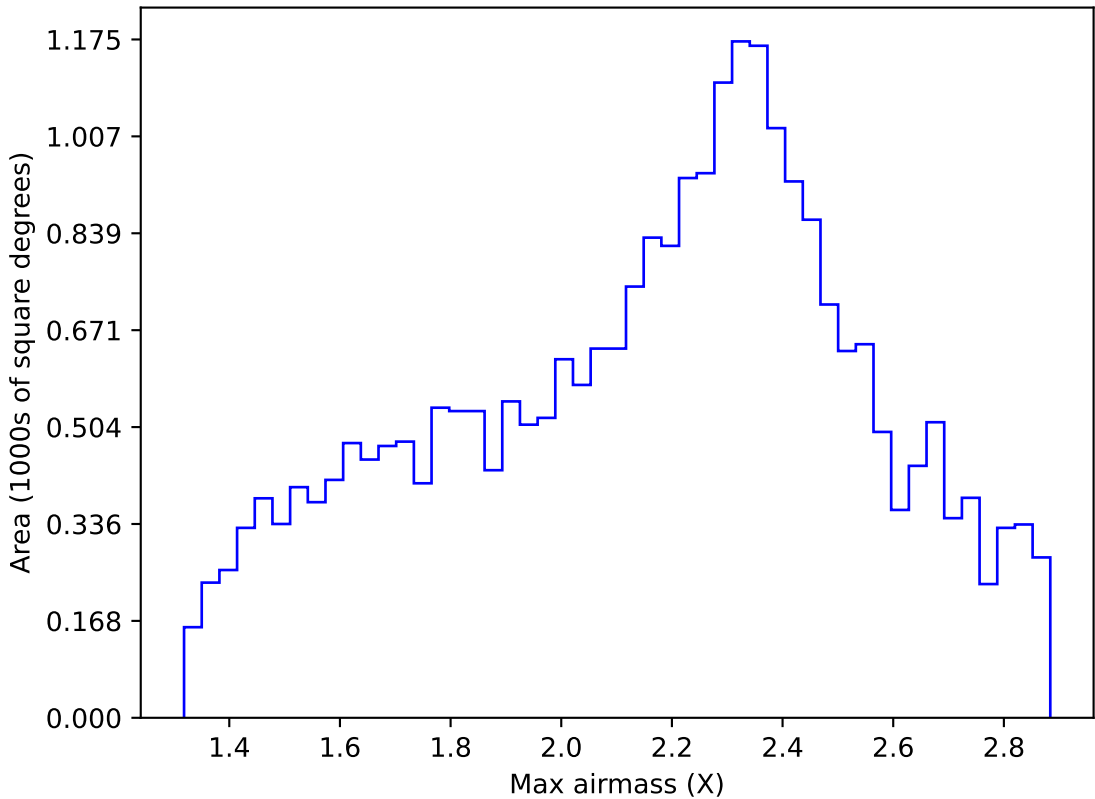
too_elab_r128_d2_griz_v3.4_10yrs Yr 1 all bands: Max airmass
