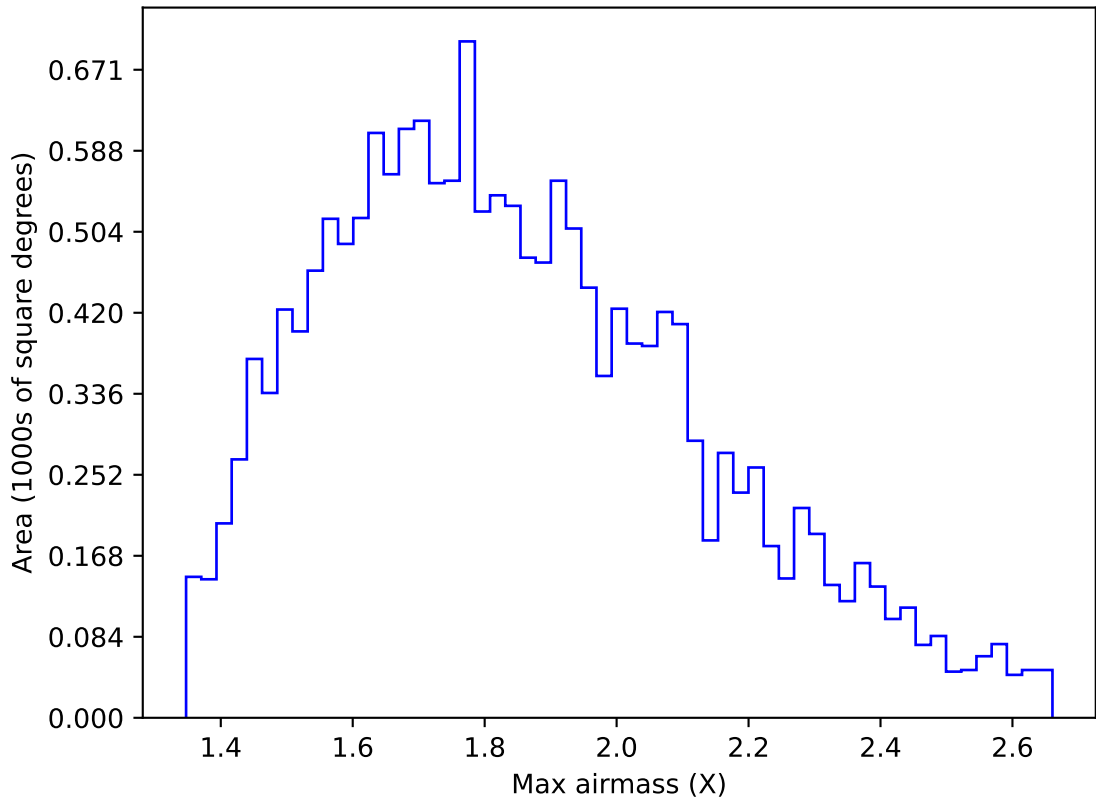
too_elab_r128_d2_griz_v3.4_10yrs WFD u band: Max airmass
