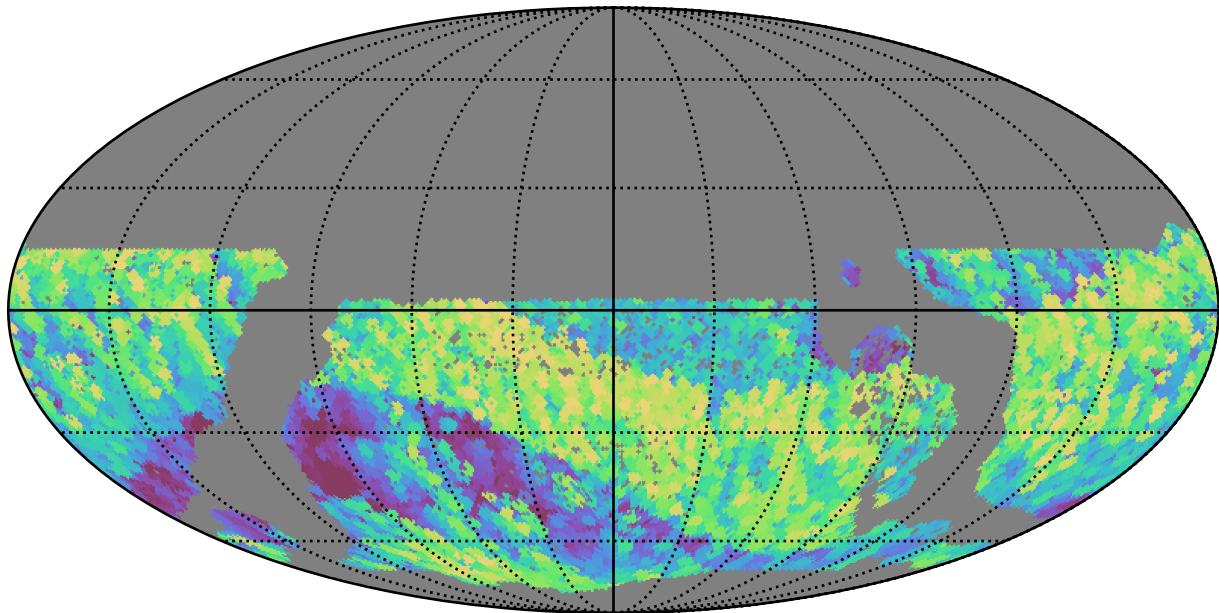
too_elab_r128_d2_griz_v3.4_10yrs WFD i band: Max airmass
