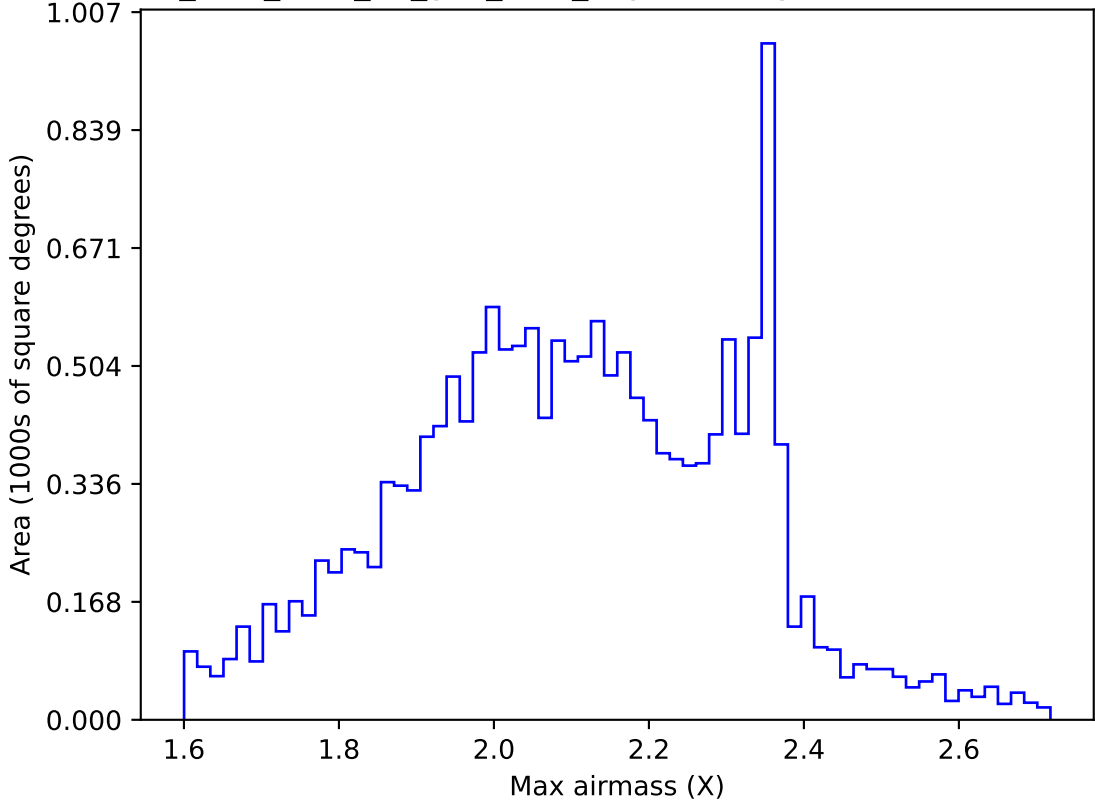
too_elab_r128_d2_griz_v3.4_10yrs WFD g band: Max airmass
