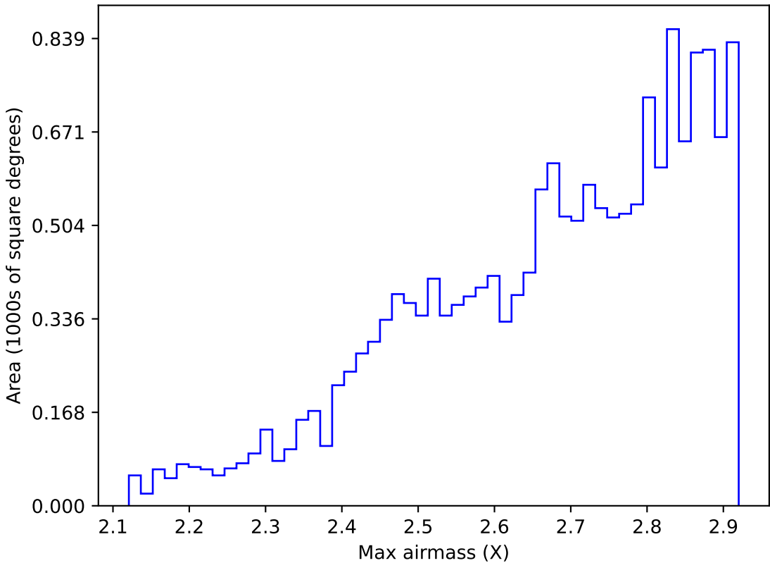
too_elab_r128_d2_griz_v3.4_10yrs WFD all bands: Max airmass
