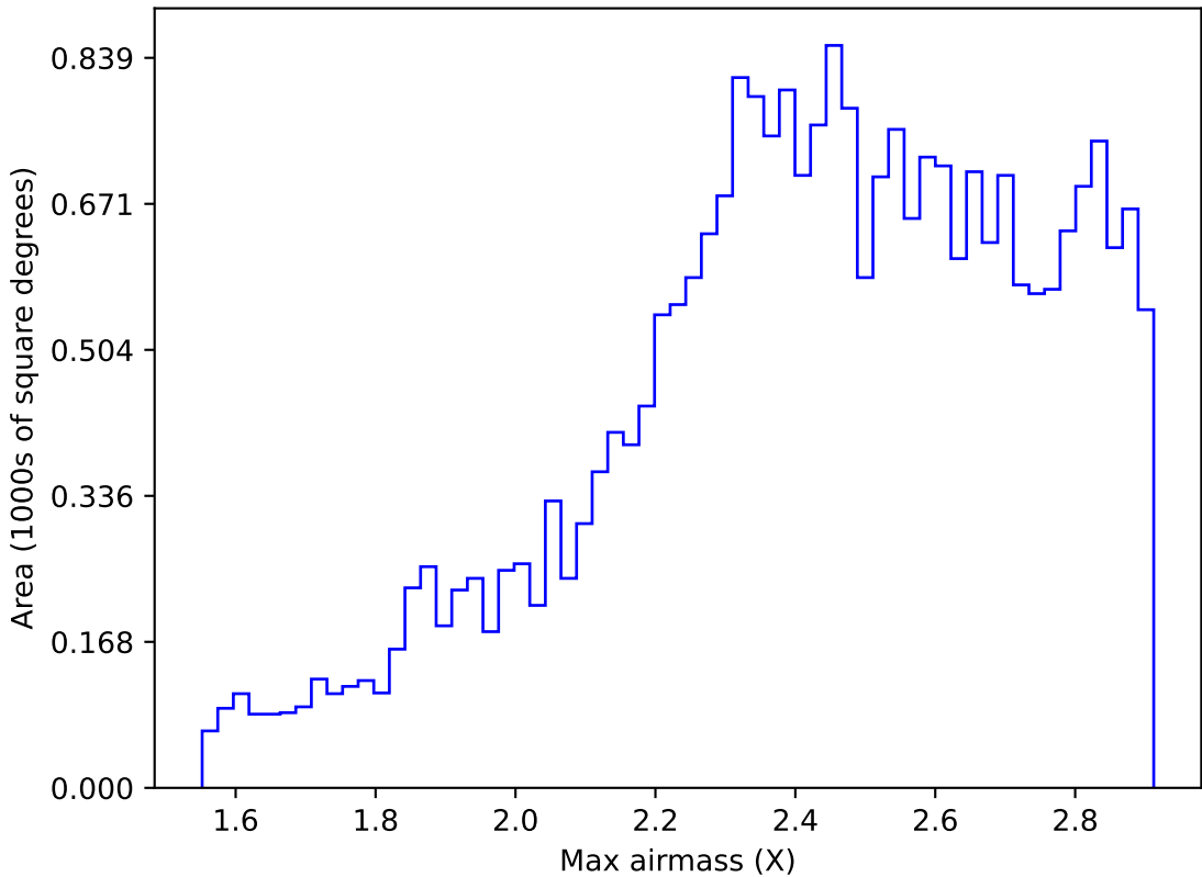
too_elab_r128_d2_griz_v3.4_10yrs All sky z band: Max airmass
