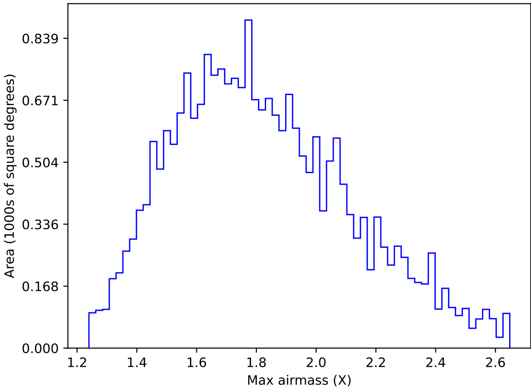
too_elab_r128_d2_griz_v3.4_10yrs All sky u band: Max airmass
