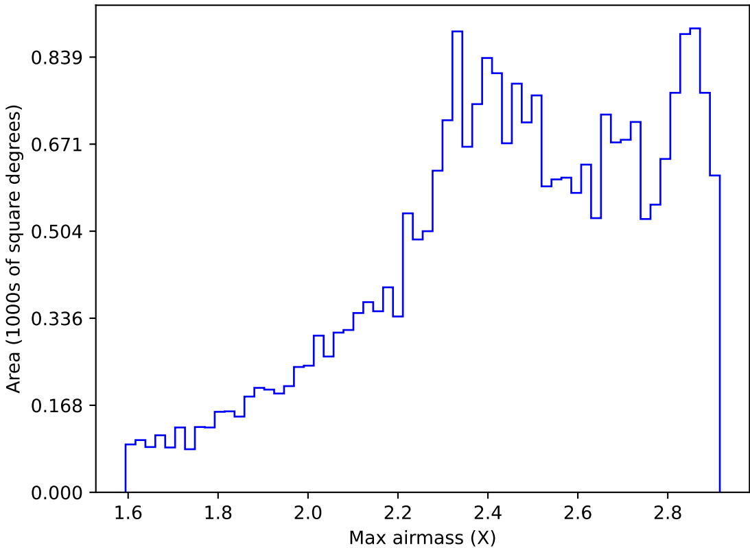
too_elab_r128_d2_griz_v3.4_10yrs All sky i band: Max airmass
