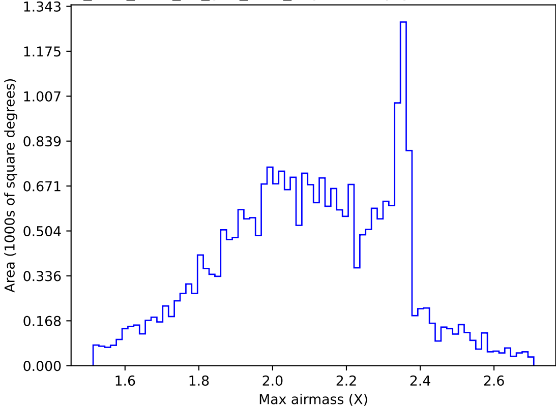
too_elab_r128_d2_griz_v3.4_10yrs All sky g band: Max airmass
