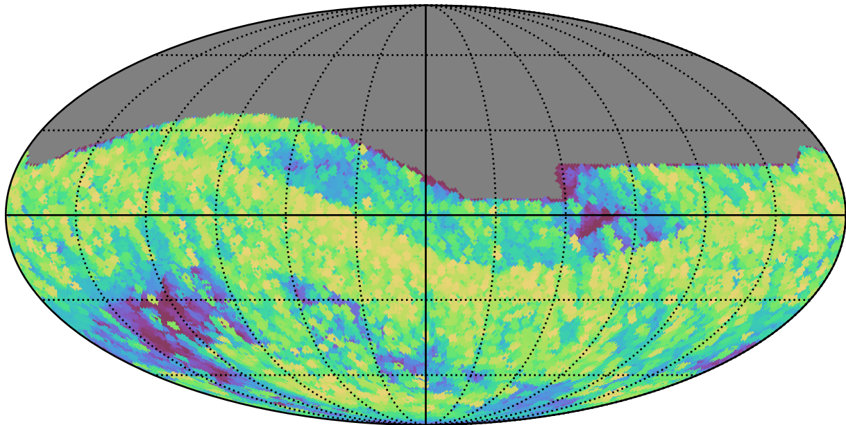
too_elab_r128_d2_griz_v3.4_10yrs All sky all bands: Max airmass
