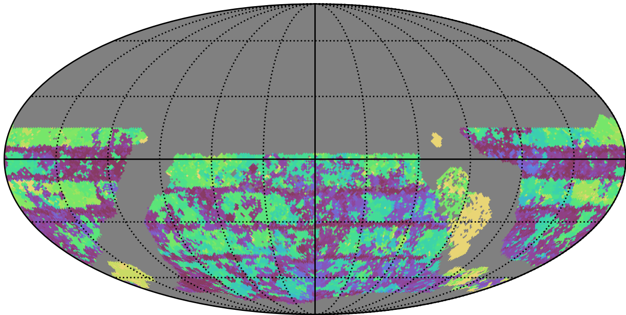
too_elab_r128_d2_griz_v3.4_10yrs WFD u band: Max Inter-Night Gap
