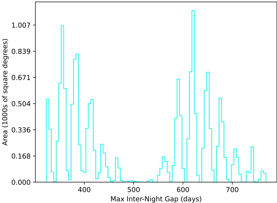
too_elab_r128_d2_griz_v3.4_10yrs WFD u band: Max Inter-Night Gap
