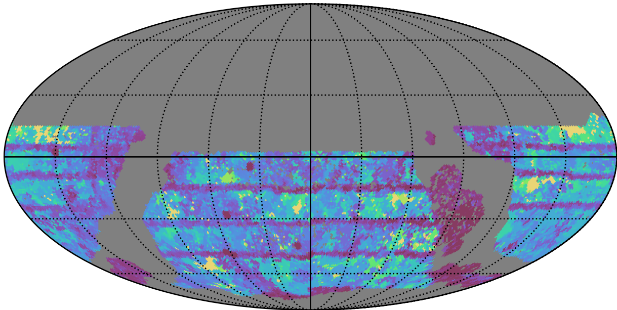
too_elab_r128_d2_griz_v3.4_10yrs WFD r band: Max Inter-Night Gap
