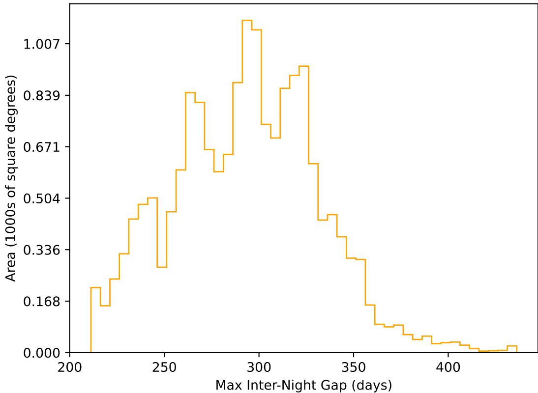
too_elab_r128_d2_griz_v3.4_10yrs WFD r band: Max Inter-Night Gap
