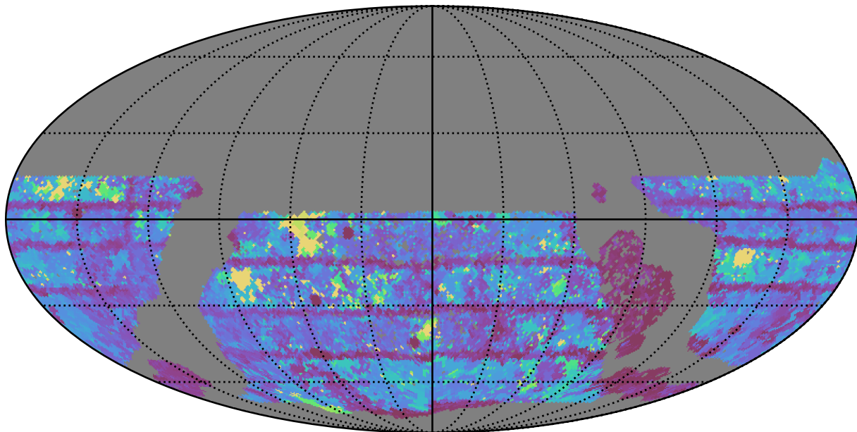
too_elab_r128_d2_griz_v3.4_10yrs WFD i band: Max Inter-Night Gap
