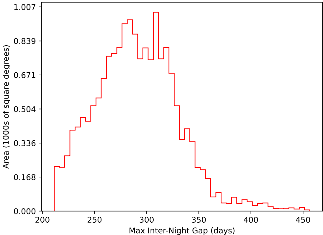
too_elab_r128_d2_griz_v3.4_10yrs WFD i band: Max Inter-Night Gap
