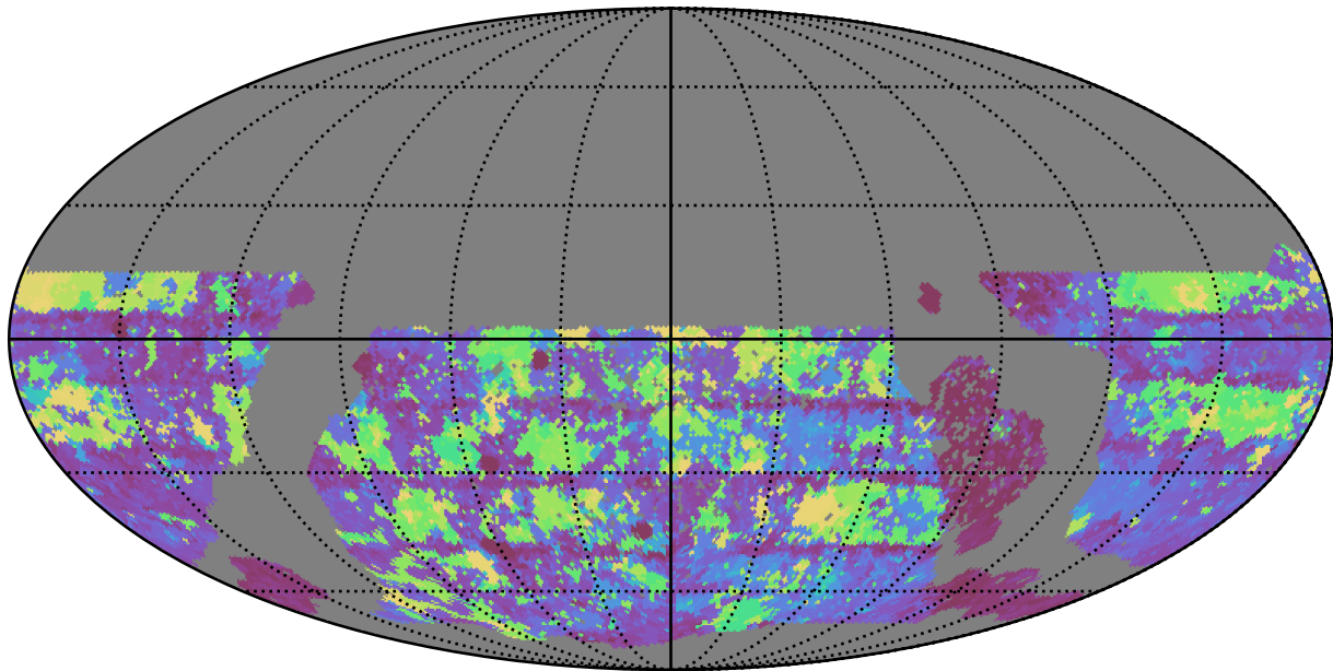
too_elab_r128_d2_griz_v3.4_10yrs WFD g band: Max Inter-Night Gap
