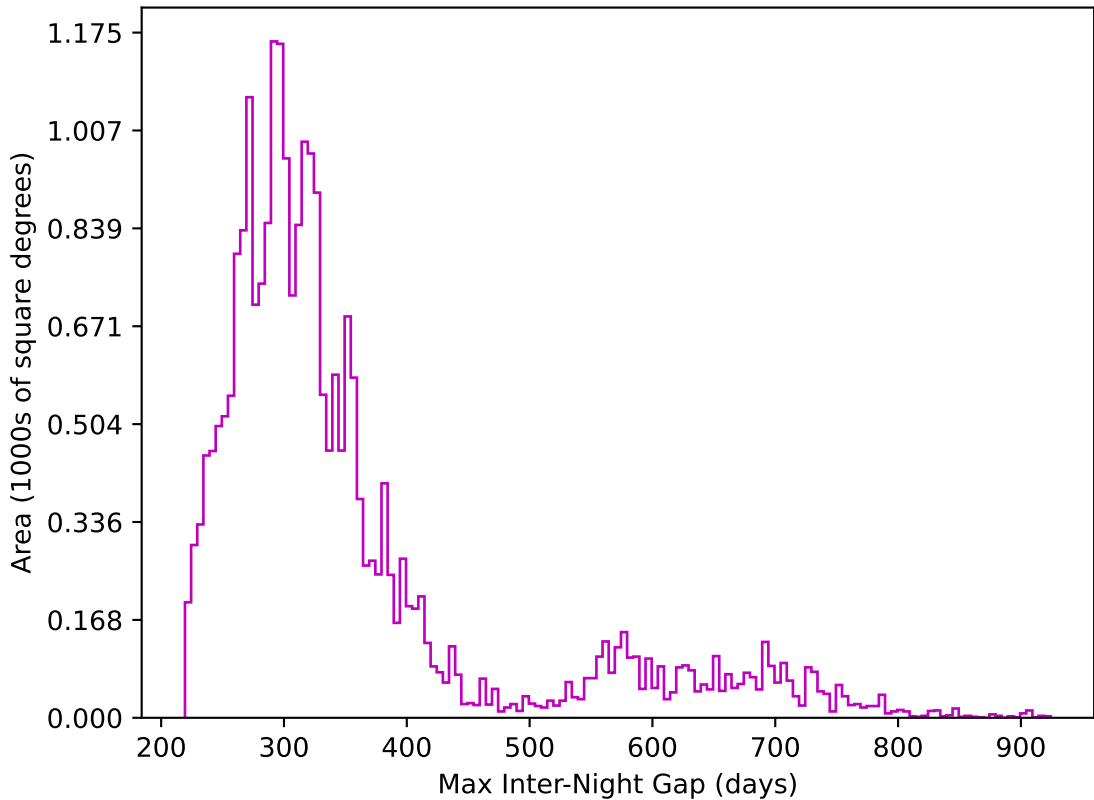
too_elab_r128_d2_griz_v3.4_10yrs All sky z band: Max Inter-Night Gap
