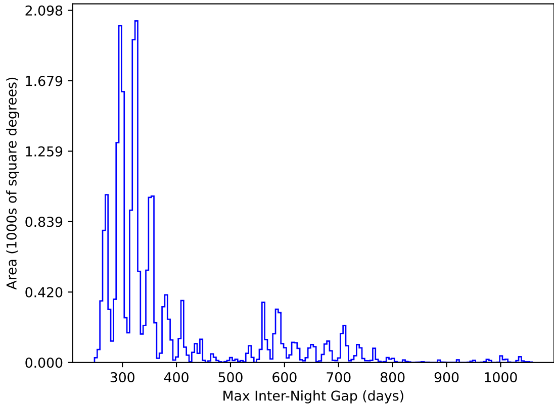
too_elab_r128_d2_griz_v3.4_10yrs All sky y band: Max Inter-Night Gap
