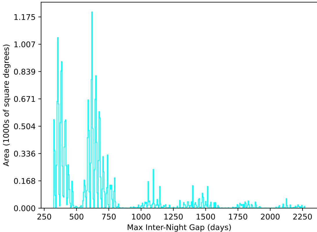
too_elab_r128_d2_griz_v3.4_10yrs All sky u band: Max Inter-Night Gap
