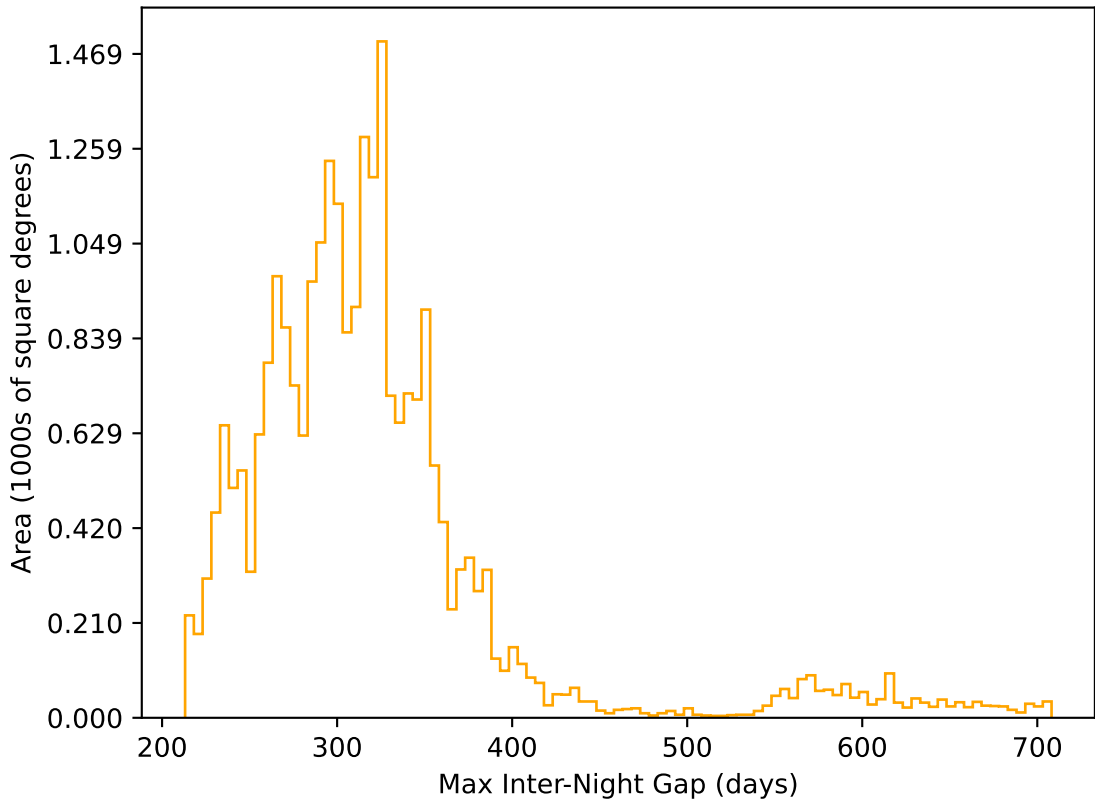
too_elab_r128_d2_griz_v3.4_10yrs All sky r band: Max Inter-Night Gap
