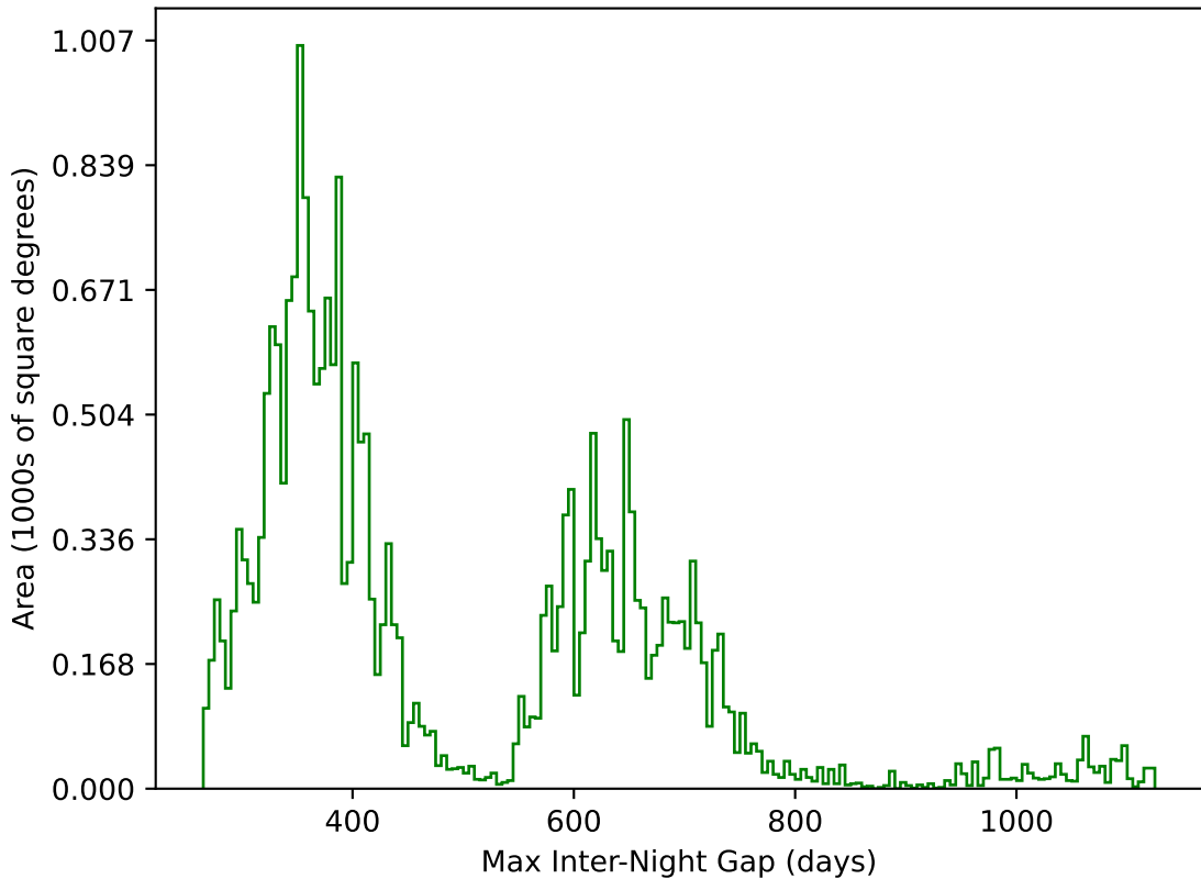
too_elab_r128_d2_griz_v3.4_10yrs All sky g band: Max Inter-Night Gap
