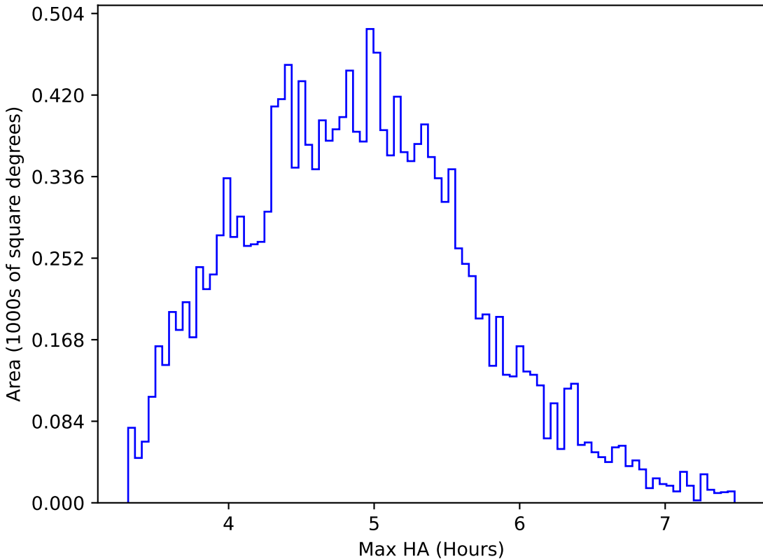
too_elab_r128_d2_griz_v3.4_10yrs WFD z band: Max HA
