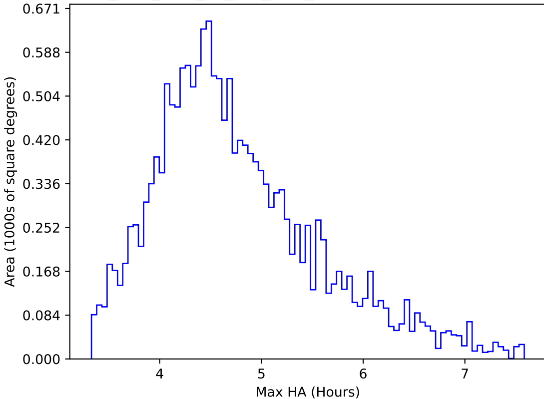
too_elab_r128_d2_griz_v3.4_10yrs WFD y band: Max HA
